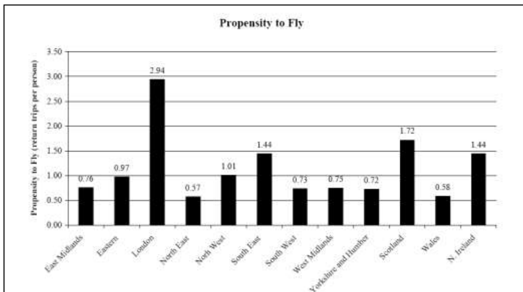
Figure 20. Propensity to fly
